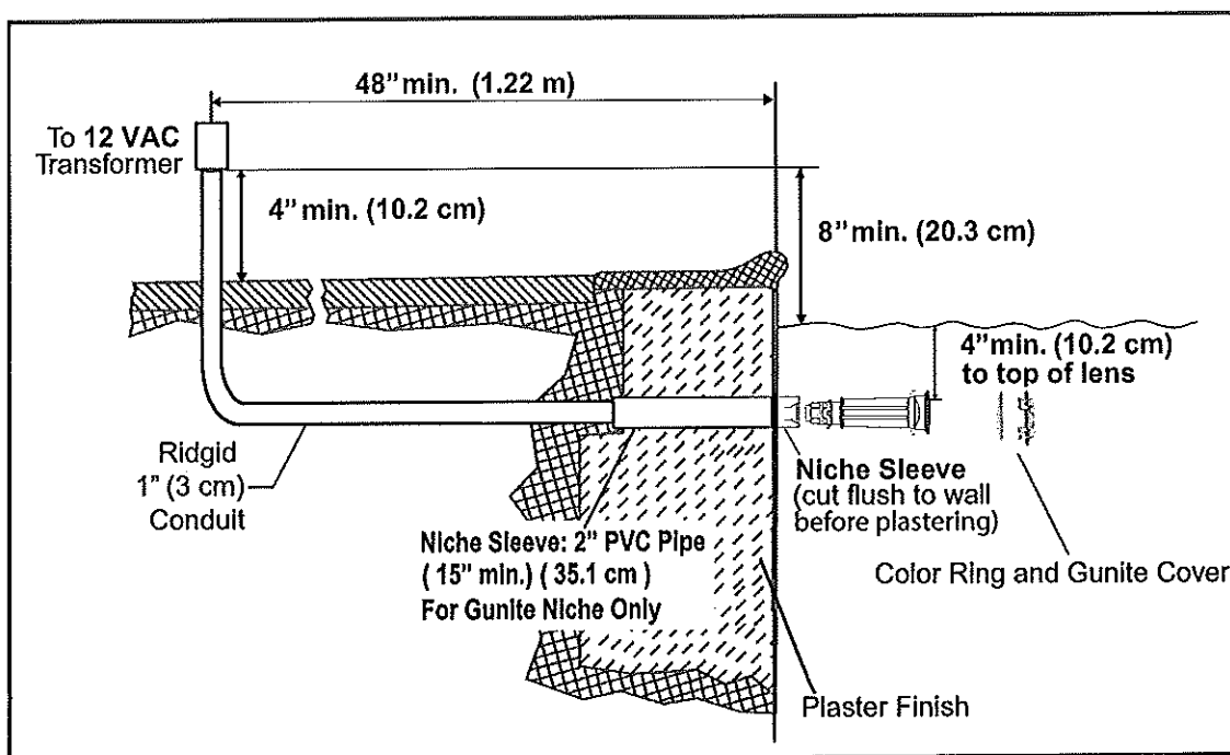
Figure 1: Gunite Light Installation Diagram
