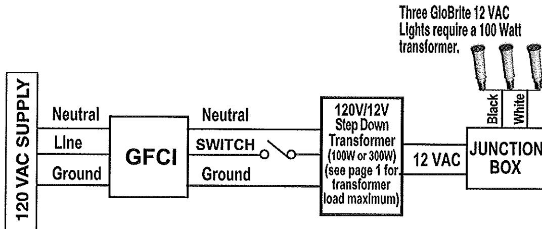
GloBrite™ Color Light with Wall Switch Wiring Diagram
