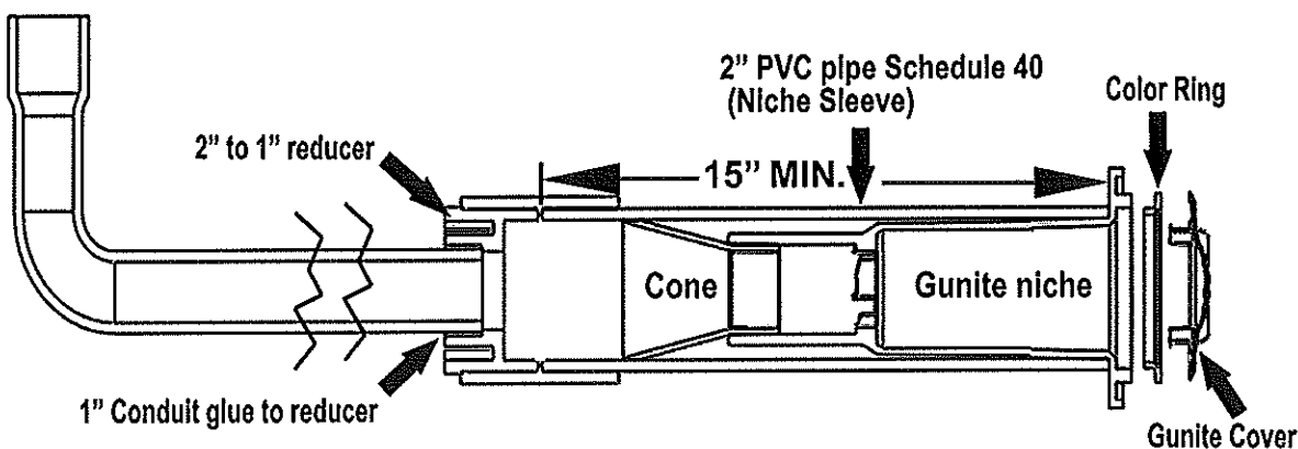
Option 1: Niche Sleeve with Cone - Installation Diagram
