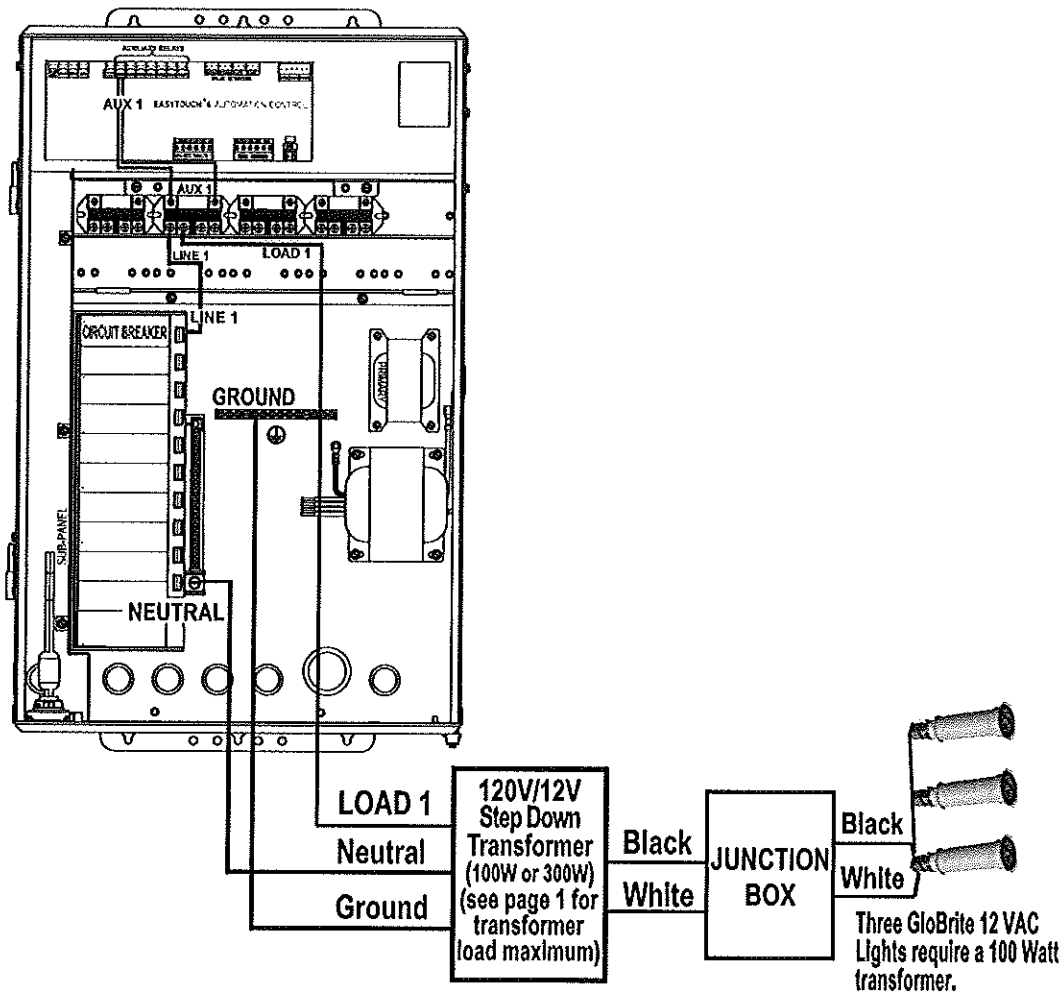
EasyTouch® and IntelliTouch® Control System Load Center Wiring Diagram
